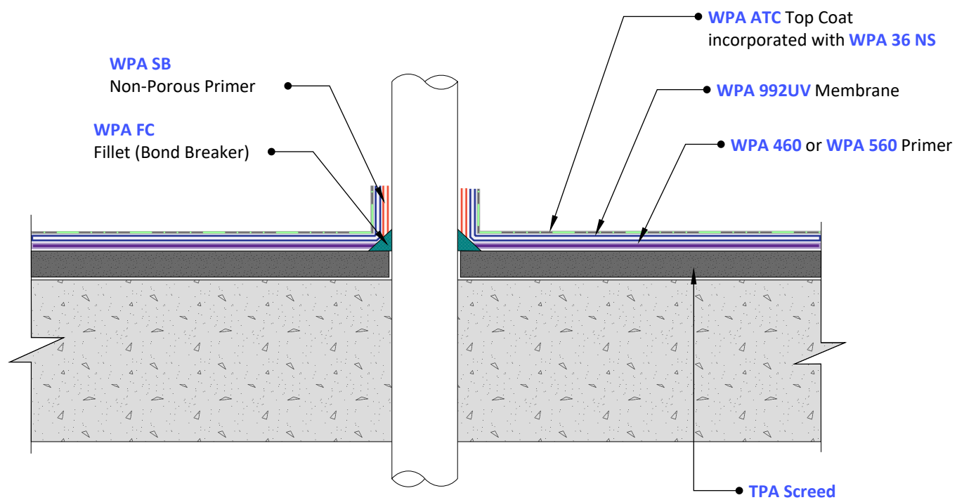
5 Pipe Penetration Scale: NTS
