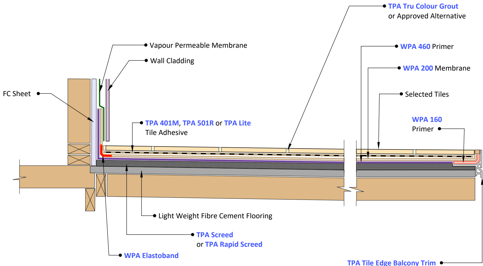
1 Floor/Wall Junction Scale: NTS
