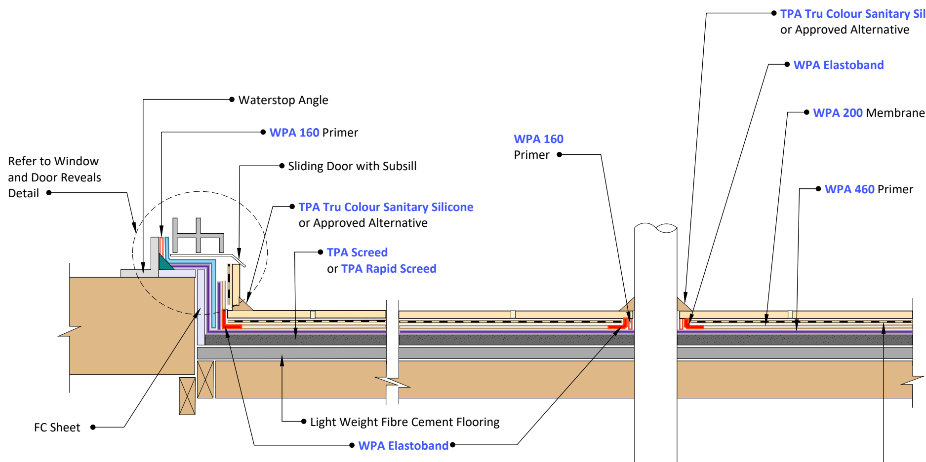
3 Sliding Door Detail Scale: NTS
