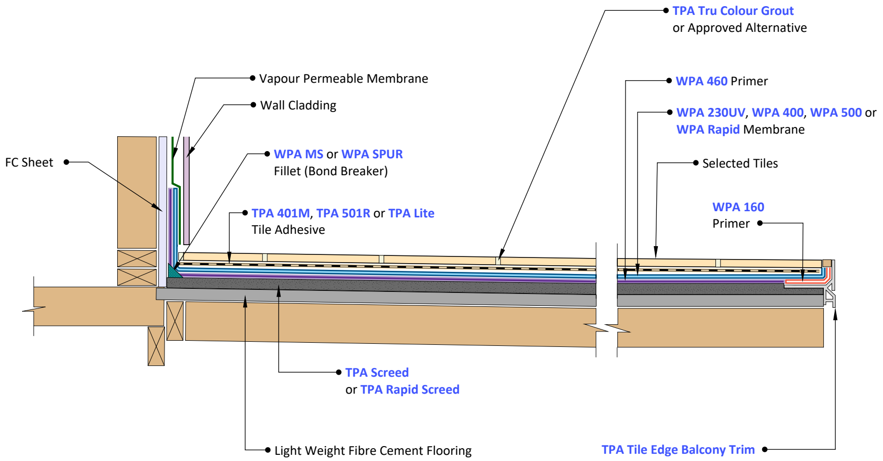
1 Floor/Wall Junction Scale: NTS
