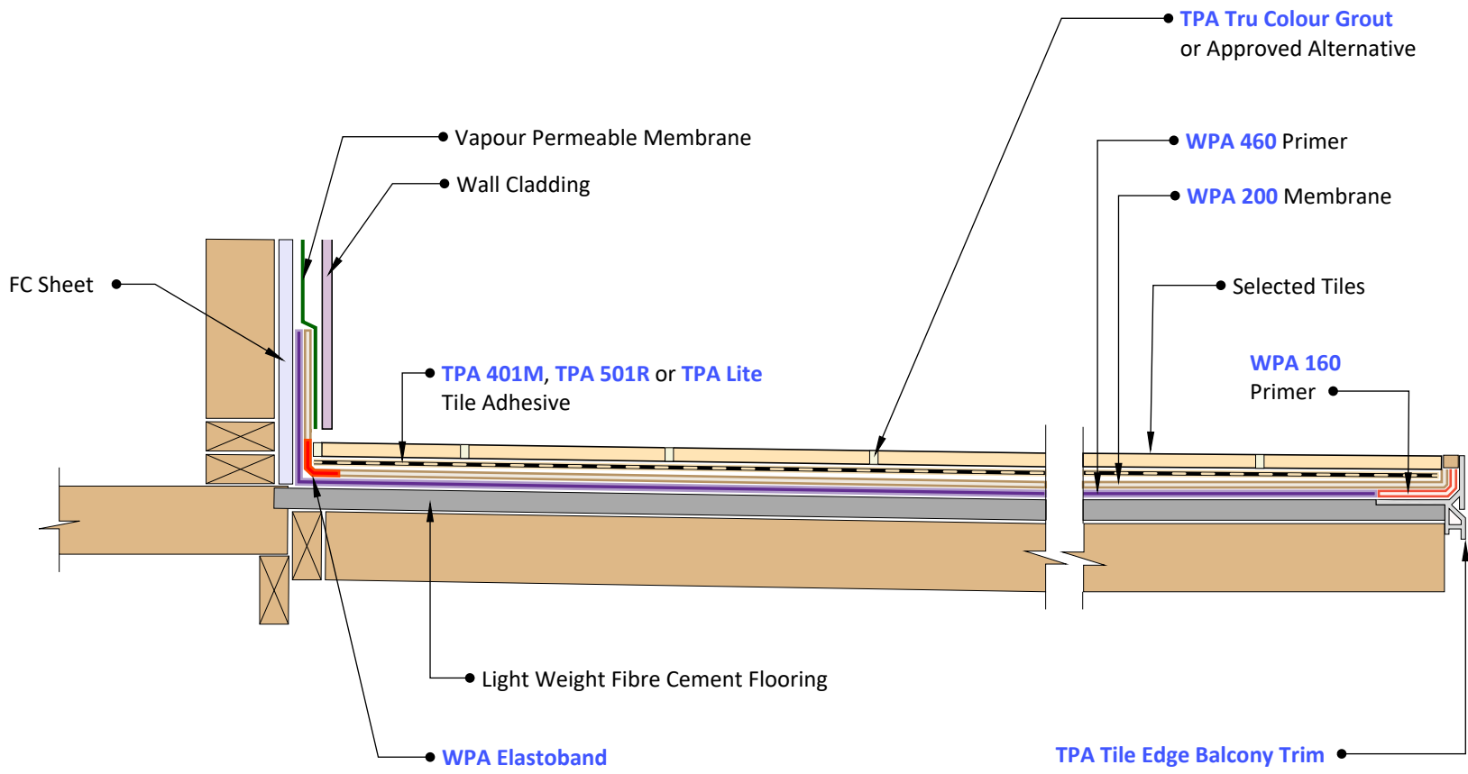
1 Floor/Wall Junction Scale: NTS
