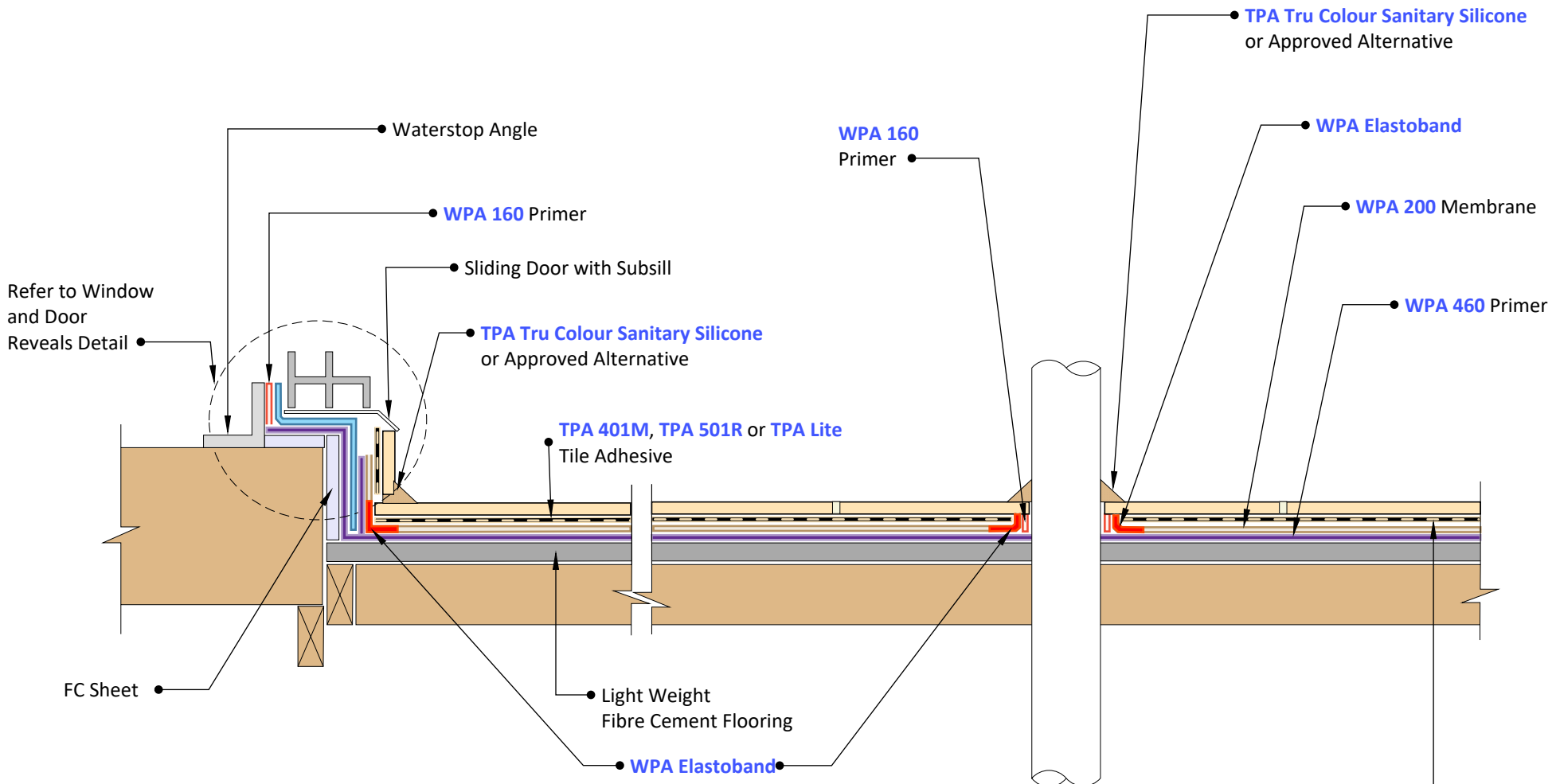
3 Sliding Door Detail Scale: NTS
